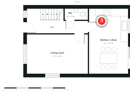
HOUSE-GROUND
